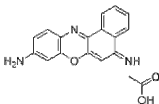
Figure 2. Structure of Cresyl Violet
