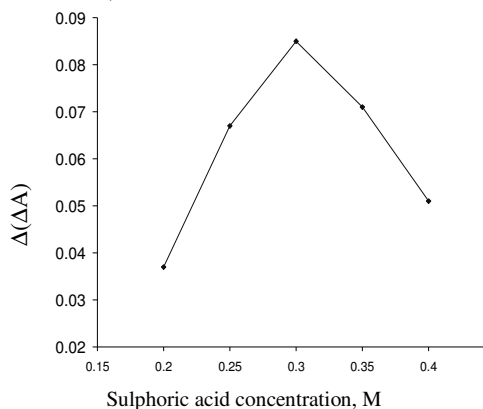
Figure 3. Effect of H_2SO_4 concentration on the analytical signal.
