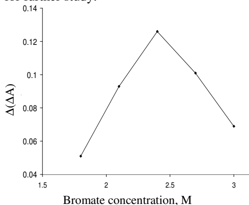
Figure 5. Influence of BrO_3^- concentration on the analytical signal.
