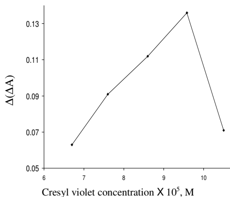
Figure 4. Effect of cresyl violet concentration on the analytical signal.
