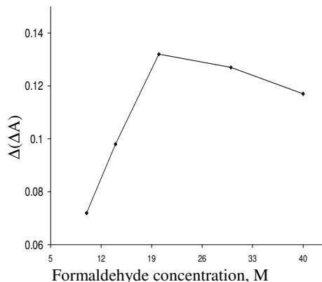
Figure 6. Influence of formaldehyde on the analytical signal.
