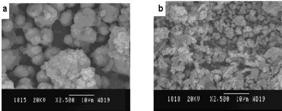
Figure 4. SEM images of (a) \text{LiMn}_2\text{O}_4 (b) \text{LiNd}_{0.3}\text{Mn}_{1.7}\text{O}_4
