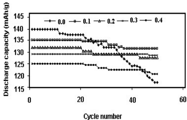
Figure 8. Plots of specific capacity vs. cycle no. of \text{LiMn}_2\text{O}_4 and \text{LiNd}_x\text{Mn}_{2-x}\text{O}_4 ( x = 0.1, 0.2, 0.3 and 0.4 )
