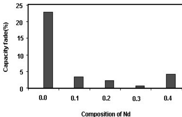
Figure 9. Capacity fading rate vs. in \text{LiMn}_2\text{O}_4 and \text{LiNd}_x\text{Mn}_{2-x}\text{O}_4 ( x = 0.1, 0.2, 0.3 and 0.4 )
