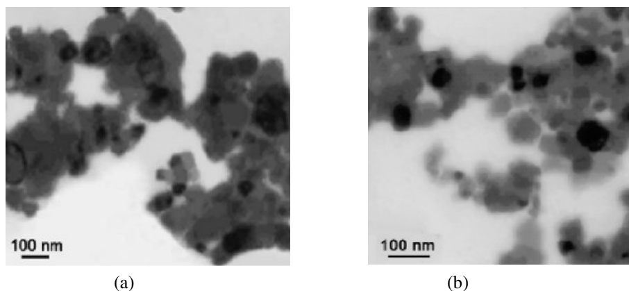
Figure 5. TEM photograph of (a) \text{LiMn}_2\text{O}_4 (b) \text{LiNd}_{0.3}\text{Mn}_{1.7}\text{O}_4
