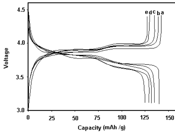
Figure 7. Charge/discharge curve of (a) \text{LiMn}_2\text{O}_4 (b) \text{LiNd}_{0.1}\text{Mn}_{1.9}\text{O}_4 (c) \text{LiNd}_{0.2}\text{Mn}_{1.8}\text{O}_4 (d) \text{LiNd}_{0.3}\text{Mn}_{1.7}\text{O}_4 and (e) \text{LiNd}_{0.4}\text{Mn}_{1.6}\text{O}_4
