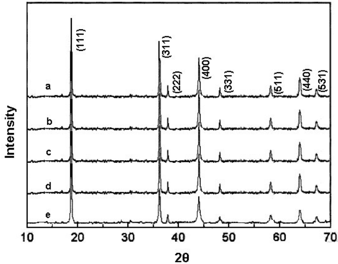
Figure 3. XRD patterns of (a) \text{LiMn}_2\text{O}_4 (b) \text{LiNd}_{0.1}\text{Mn}_{1.9}\text{O}_4 (c) \text{LiNd}_{0.2}\text{Mn}_{1.8}\text{O}_4 (d) \text{LiNd}_{0.3}\text{Mn}_{1.7}\text{O}_4 and (e) \text{LiNd}_{0.4}\text{Mn}_{1.6}\text{O}_4
