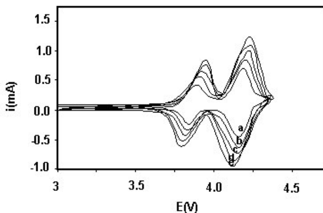
Figure 6. Cyclic voltammetry curve of (a) \text{LiMn}_2\text{O}_4 (b) \text{LiNd}_{0.1}\text{Mn}_{1.9}\text{O}_4 (c) \text{LiNd}_{0.2}\text{Mn}_{1.8}\text{O}_4 (d) \text{LiNd}_{0.3}\text{Mn}_{1.7}\text{O}_4 and (e) \text{LiNd}_{0.4}\text{Mn}_{1.6}\text{O}_4
