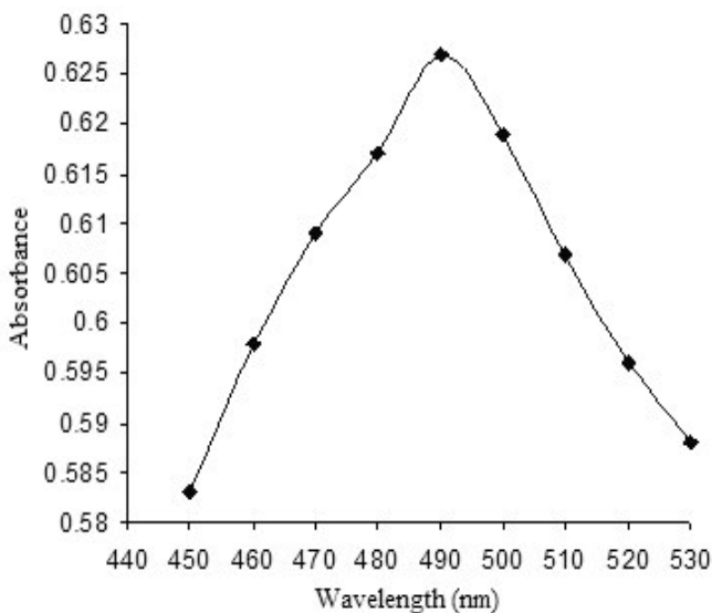
Figure 4. Absorption spectrum of the azo dye formed between AFZ (10 µg/mL) and acetyl acetone
