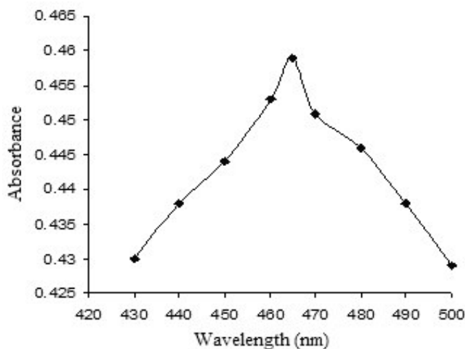
Figure 3. Absorption spectrum of the azo dye formed between AFZ (10 \mu g/mL) and ethylcyanoacetate
