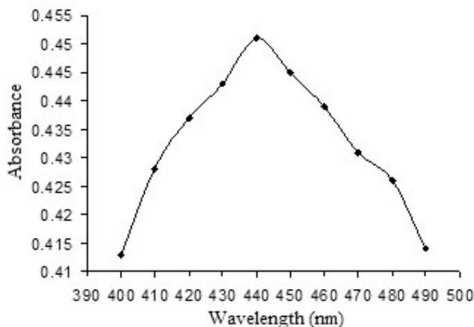
Figure 2. Absorption spectrum of the azo dye formed between AFZ (10 \mu g/mL) and ethoxyethylenemaleic ester
