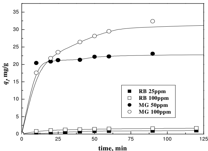
Figure 3. Kinetic curves for the adsorption of dyes on TFC
