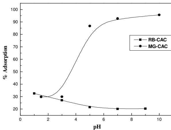
Figure 2. Effect of pH on the adsorption of RB and MG
