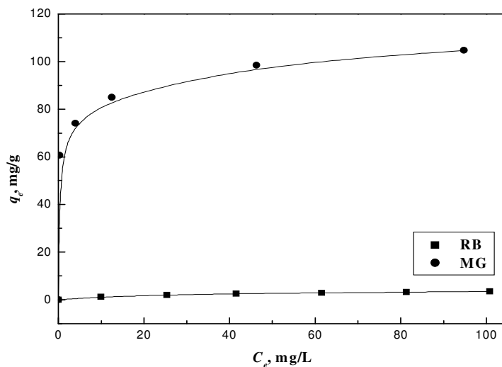
Figure 1. Adsorption of RB and MG on TFC
