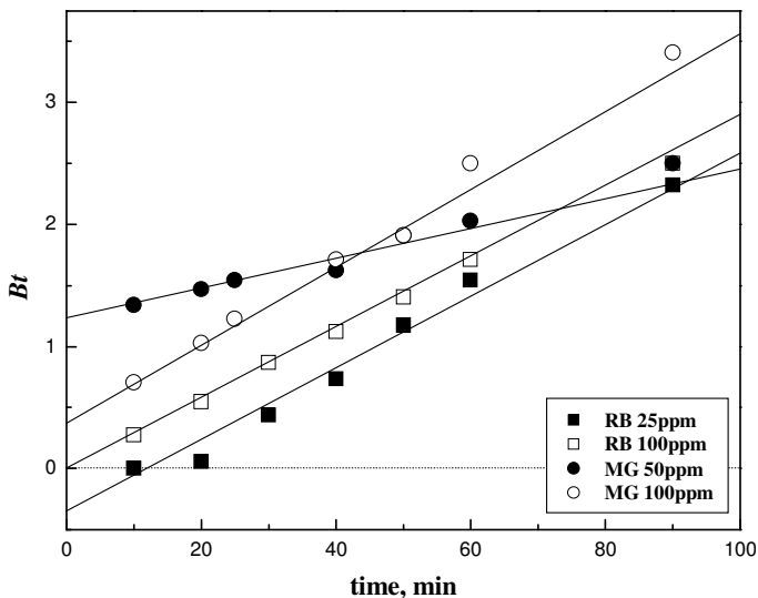
Figure 4. t versus Bt plots for the adsorption of dyes at different concentrations
